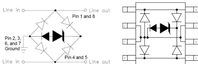
Circuit and Pin Schematic
