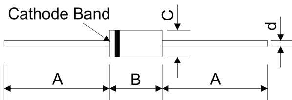
DO-201
